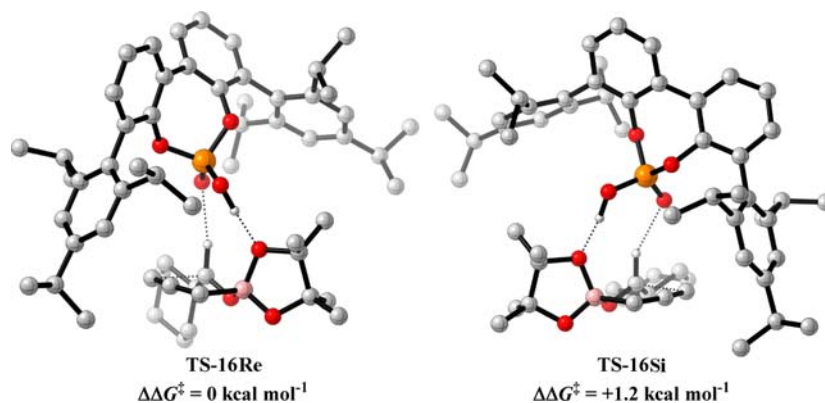
Figure 6. Competing TS for the reaction of cyclohexanecarboxaldehyde and allenylboronic acid pinacol ester catalyzed by ( R )-3,3'-bis(2,4,6-triisopropylphenyl)-1,1'-bi-2-phenol-phosphoric acid. Geometries B3LYP/6-31G*, single-point energies M06-2X/6-31G*. Noncritical hydrogen atoms omitted for clarity.
