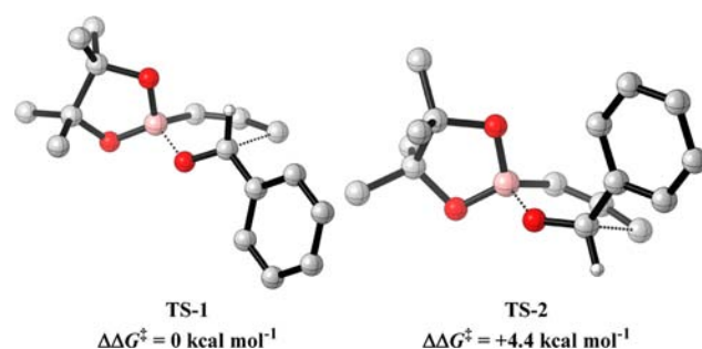
Figure 1. Competing TS for the reaction of benzaldehyde and allenylboronic acid pinacol ester. Geometries B3LYP/6-31G*, single-point energies M06-2X/6-31G*. Noncritical hydrogen atoms omitted for clarity.
