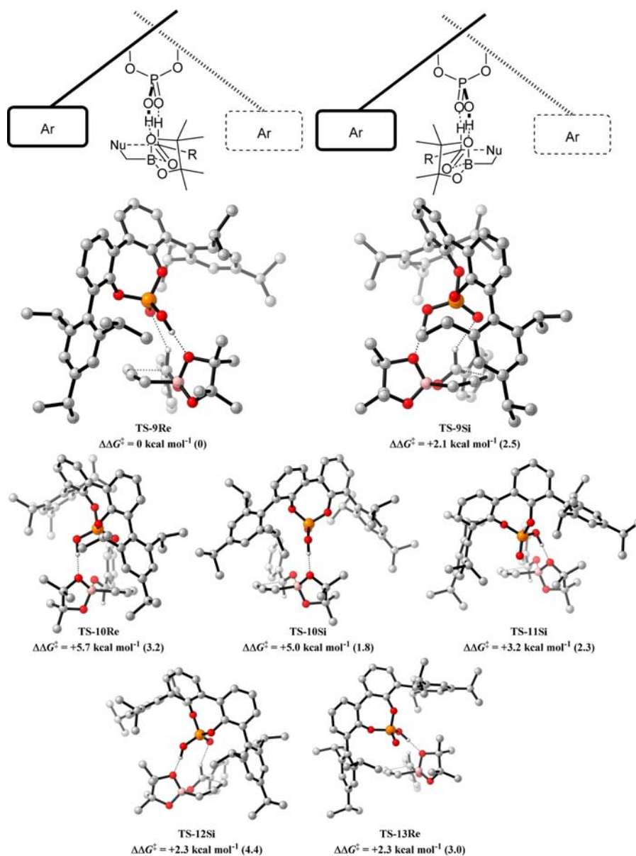
Figure 3. Competing TS for the reaction of benzaldehyde and allenylboronic acid pinacol ester catalyzed by ( R )-3,3'-bis(2,4,6-triisopropylphenyl)-1,1'-bi-2-phenol-phosphoric acid. Geometries B3LYP/6-31G*, single-point energies M06-2X/6-31G*. B3LYP/6-31G* free energies in parentheses. Noncritical hydrogen atoms omitted for clarity.
