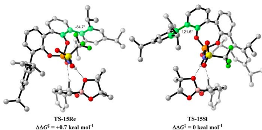
Figure 5. Competing TS for the reaction of benzaldehyde and allenylboronic acid pinacol ester catalyzed by a BINOL-derived N -triflyl phosphoramidate. Geometries B3LYP/6-31G*, single-point energies M06-2X/6-31G*. Measured dihedrals highlighted in green. Noncritical hydrogen atoms omitted for clarity.
