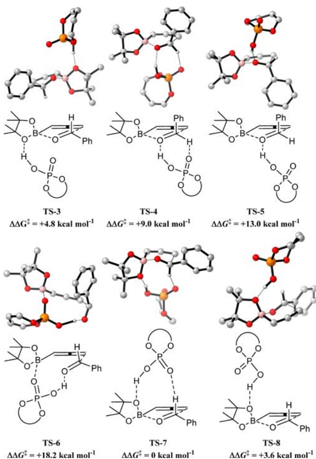
Figure 2. Competing TS for the reaction of benzaldehyde and allenylboronic acid pinacol ester catalyzed by buta-1,3-diene-1,4-diol-phosphoric acid. Geometries B3LYP/6-31G*, single-point energies M06-2X/6-31G*. Noncritical hydrogen atoms omitted for clarity.
