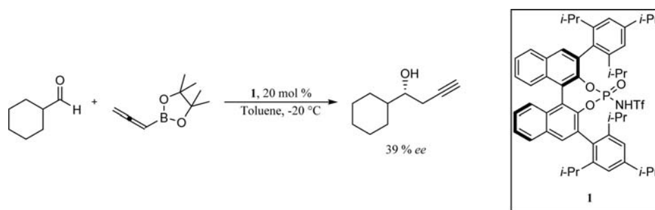
Figure 7. Reaction of cyclohexanecarboxaldehyde and allenylboronic acid pinacol ester catalyzed by 1 .
