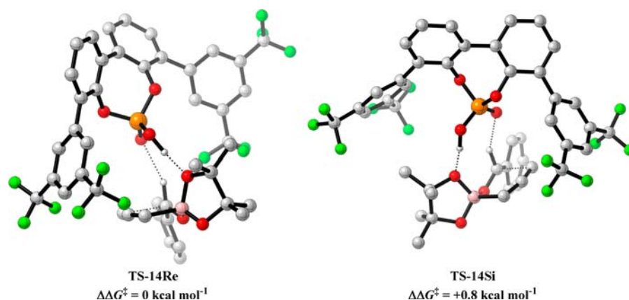
Figure 4. Competing TS for the reaction of benzaldehyde and allenylboronic acid pinacol ester catalyzed by ( R )-3,3'-bis(3,5-bis(trifluoromethyl)phenyl)-1,1'-bi-2-phenol-phosphoric acid. Geometries B3LYP/6-31G*, single-point energies M06-2X/6-31G*. Noncritical hydrogen atoms omitted for clarity.
